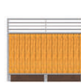
Standard plus fence elements: Height 1,60 m
